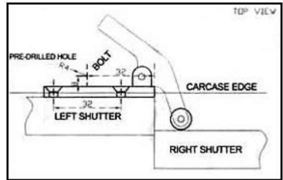
Installation Diagram
