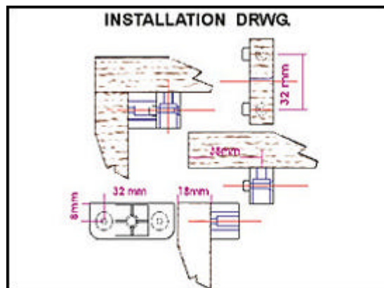
Installation Diagram
